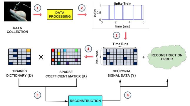
Figure 1: The proposed dictionary learning framework for neuronal signal modeling. (1) Data is acquired. (2) Action potentials are transformed to binary values. (3) Data is represented in matrix format. (4) Dictionary learning is applied on the training data. (5) Testing examples are represented by a linear combination of a few dictionary elements. (6) Reconstruction error is quantified.
