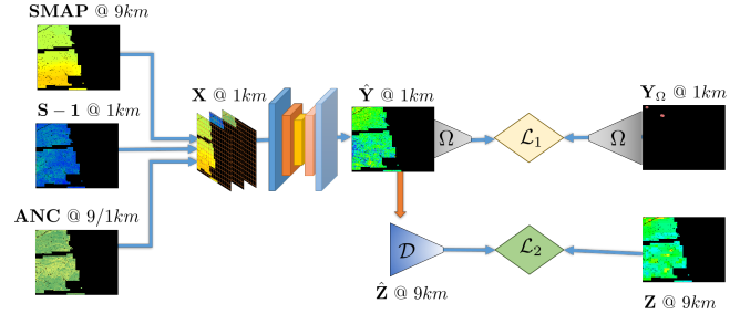
Fig. 1. Block diagram of the proposed framework: Remote sensing observations from SMAP at 9 km, Sentinel 1 at 1 km, and ancillary measurements are incorporated into the CNN model. The model initially produces high spatial resolution SSM estimations and subsequently generates a lower-resolution version.
