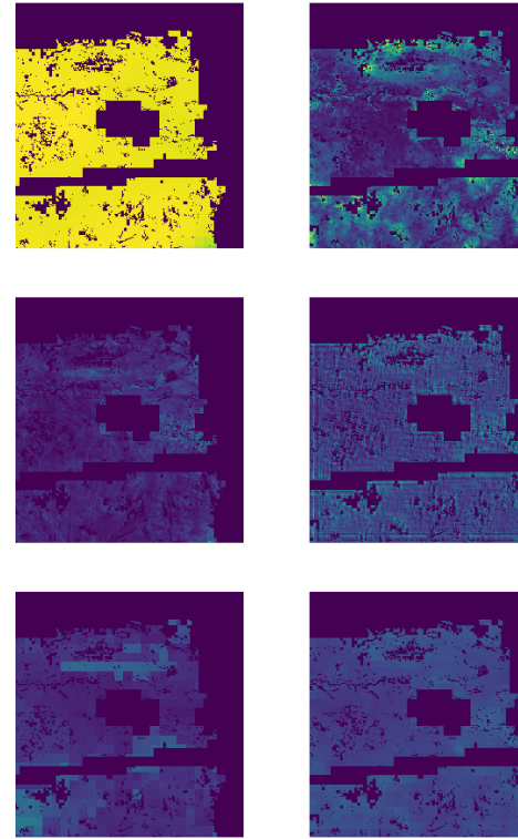
Fig. 3. Visualization of input data (top row), SSM estimates at fine resolution (middle row), and SSM estimates at coarse resolution (bottom row).
