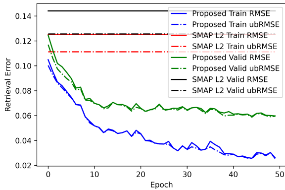
Fig. 2. Retrieval error (RMSE and ubRMSE) for the proposed model as a function of training epoch. The enhanced SMAP/Sentinel 1 L2 product at 1 km is also included for reference.
