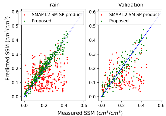
Fig. 4. Scatter plot of retrieval SSM against in situ measurements for the proposed and the SMAP L2 product.
