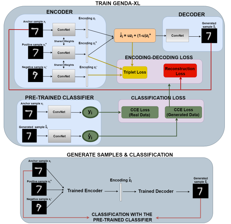
Fig. 1: Proposed generative model GENDA-XL
