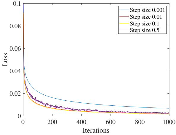
Fig. 2. Convergence behavior of the proposed method for varying gradient step sizes.
