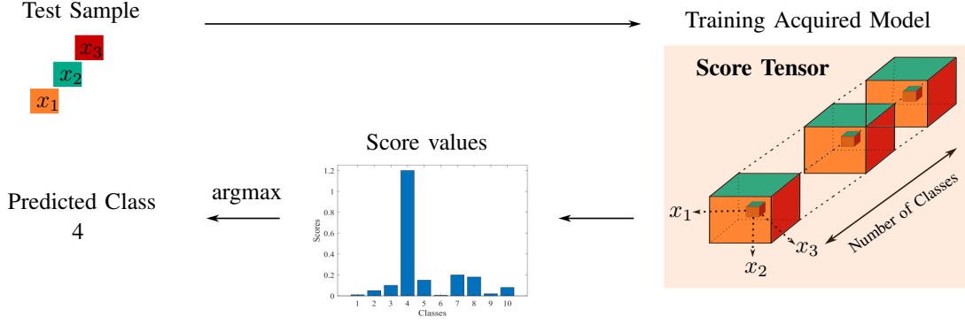
Fig. 1. Flowchart depicting the steps involved in the proposed classification method. To classify a new sample, we extract the scores that correspond to the last dimension of the learned tensor at the position specified by the sample value. The predicted class for the sample is the one associated with the highest score.
