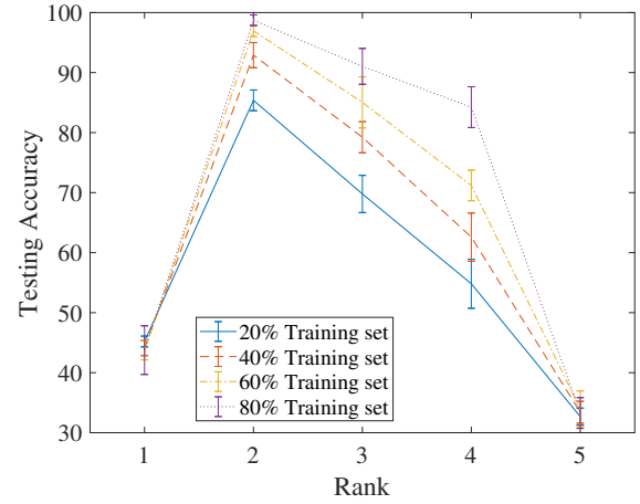
Fig. 3. Evaluation of testing accuracy across various multi-linear ranks of the score tensor and different training set sizes.
