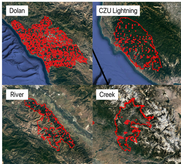
Fig. 2. Burned area mapped using CYGNSS and XGBoost for largest fires in 2020. Red dots indicate burning predicted by ML model and the red boundary is the burn perimeter from the Cal Fire dataset.
