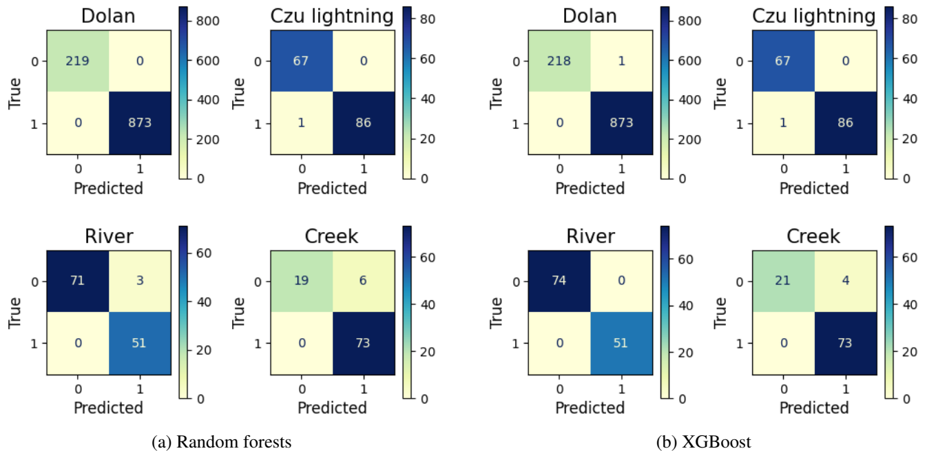
Fig. 3. Confusion matrices of the largest four fires in California in 2020 with coverage from CYGNSS using two ML models.
