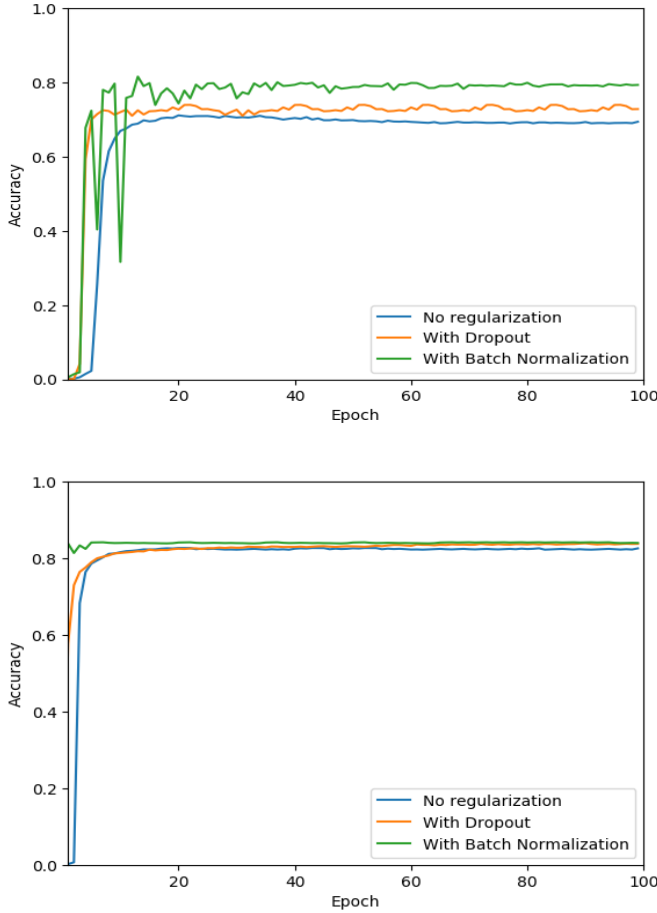
Fig. 12. Impact of regularization, in regard with the size of the training set. In the upper plot, a network trained with 400,000 observations is illustrated, while in the lower plot 4,000,000 training examples have been utilized.
