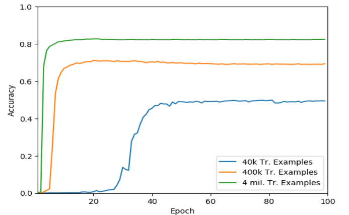
Fig. 10. Accuracy on the Validation Set for different sizes of the Training Set. No regularization has been used.
