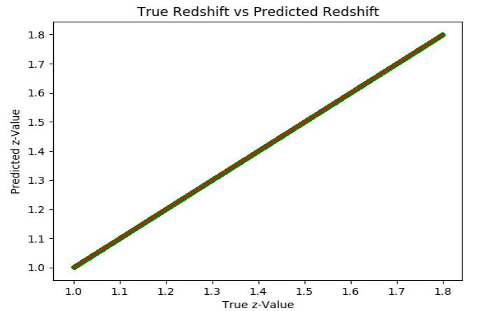
Fig. 7. Performance of a 3-Layered network trained with 400,000 training examples. In the first plot we compare the cases where the redshift estimation problem is transformed into a classification task, with the use of 800 versus 1600 classes. In the second plot, we present the scatter plot of the predicted result versus the state-of-nature of the testing samples, only for the case of 1600 total classes.
