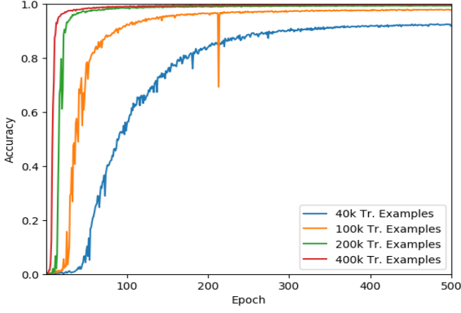
Fig. 6. Validation performance of a 3-layered network, using larger and more limited in size datasets. In all cases the training accuracy (not depicted here) can asymptotically reach 100% accuracy, after enough epochs.
