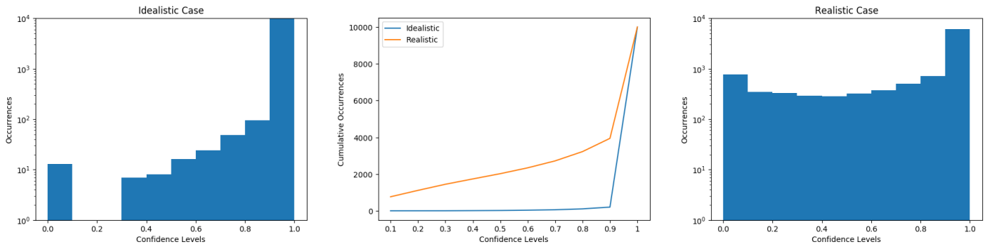
Fig. 14. Levels of confidence derived by softmax in the testing set. The middle plot depicts the cumulative occurrences per level of confidence, for both examined cases. For example, the y-axis value that corresponds to the x-value of 0.4, represents the number of testing observations that obtain a predictive output from the trained model with a confidence that is less than or equal to 0.4. The left (idealistic case) and right (realistic case) histograms, exhibit a similar scenario, but not in a cumulative form (and in logarithmic scale).
