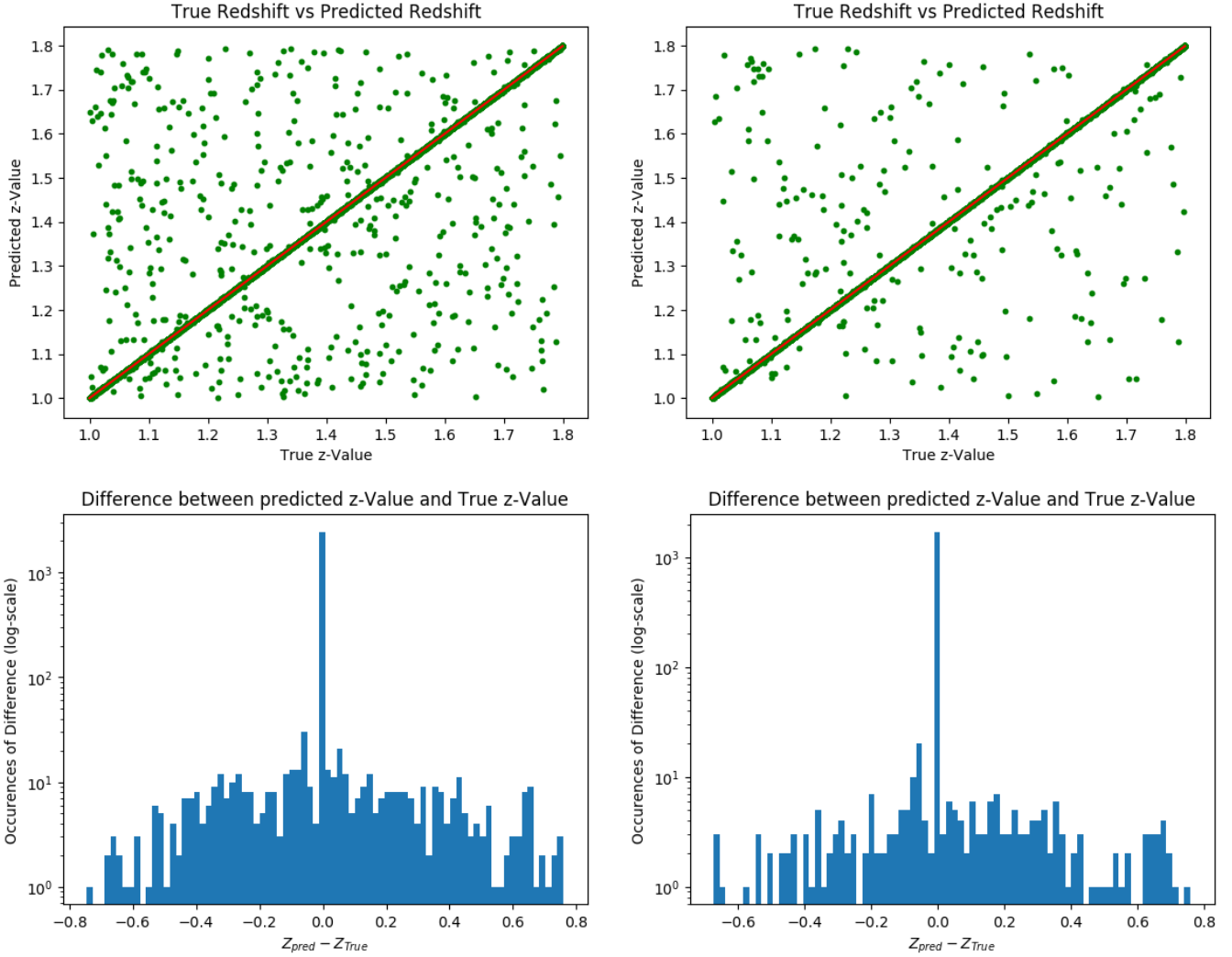
Fig. 11. Classification scatter plots & histograms for the realistic case, for 3-layered networks trained with 400,000 Training Examples (column a) & 4,000,000 Training Examples (column b). The depicted histograms, represent the actual difference in distance (positive or negative) between misclassified estimated values and their corresponding ground truth value versus the frequency of occurrence, in logarithmic scale, for each case.
