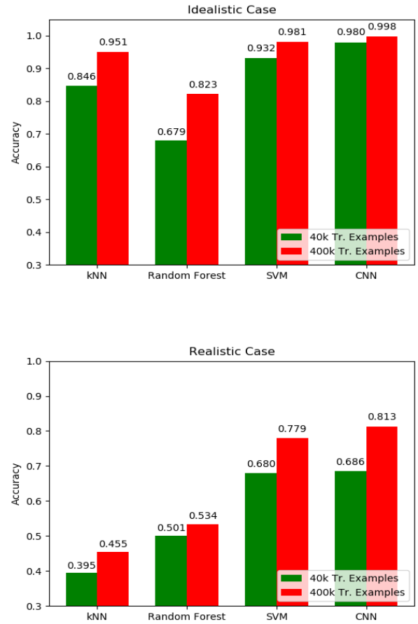
Fig. 13. Comparison bar plots for the k Nearest Neighbours, Random Forest, Support Vector Machines and Convolutional Neural Networks algorithms. We present the best case performance on the test set, for each classifier, in the idealistic and the realistic case, with a limited and an increased amount of training data.
