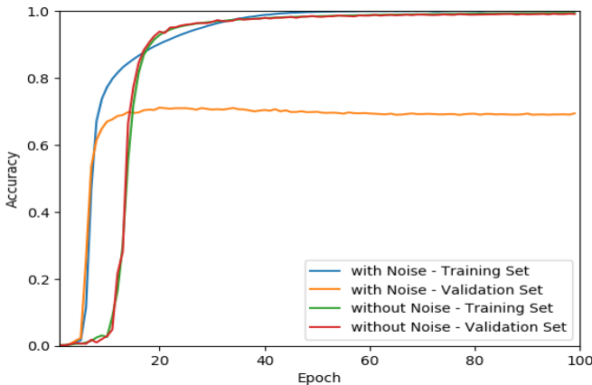
Fig. 9. Comparison of the model's performance, trained with clean and with noisy data (400,000 in both cases). The 3-layered neural network utilizes the same hyperparameters, in both cases, without any form of regularization.
