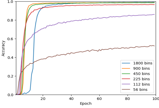
Fig. 8. Validation performance of a 3-Layered network trained with 400,000 training examples. We want to examine the behavior of the model, when trained with data of reduced dimensionality.
