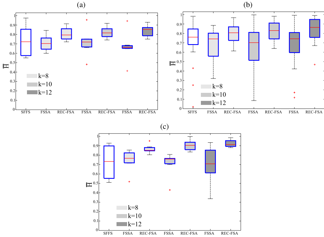
Fig. 13. The \bar{H} value for the resulting reduced set f_{ij}^* , for all cases of WSN deployments when the link performance: is (a) problematic, (b) good, and (c) excellent.
