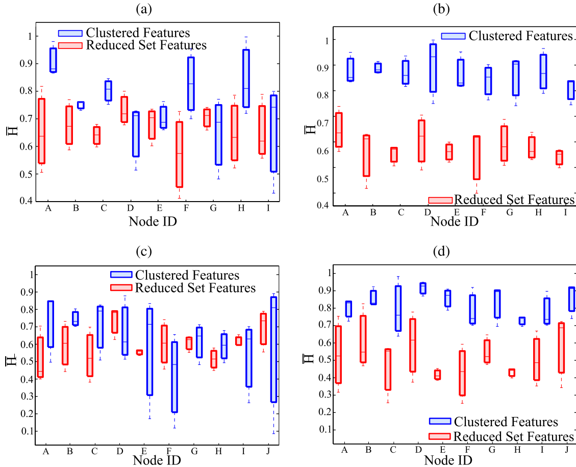
Fig. 14. The \bar{H} of f_{ij}^* and the c_m /sensor node for both cases of rural (top) and industrial (bottom) deployments (Stack 1 and Stack 2), when FSSA ((a) and (c)) and REC-FSA ((b) and (d)) are applied ( k=12 ).
