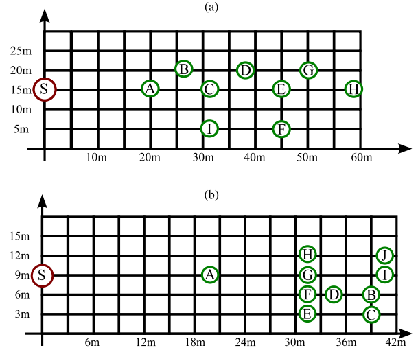
Fig. 7. The layout of the WSN deployments at (a) the rural (a), and (b) the industrial environments.
