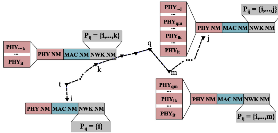
Fig. 5. A data-flow example over path P_{ij} , highlighting the piggy-backing process for updating the contents of the NM preamble.
