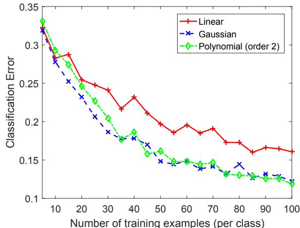
Figure 4: Classification error as a function of training examples using 20 frames per sequence, where only spatial features are extracted by the VGG-16 network for three SVM kernels.
