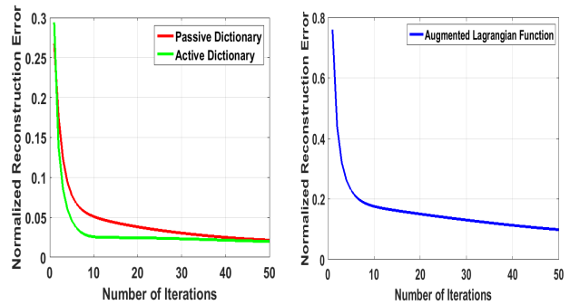
Figure 5: (a) Convergence Behaviour of the ADMM coupled dictionary learning Algorithm, (b) Convergence of the augmented Lagrangian function. The number of dictionary atoms was fixed to 512, while we used a (3 \times 3) patch size. We observe that the coupled dictionaries and the augmented Lagrangian function converge into a stationary point after approximately 10 iterations.
