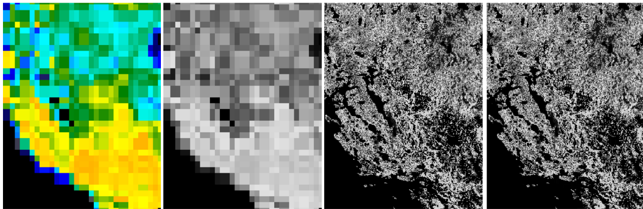
(a) Input Passive California (RGB) (b) Input Passive California (c) Ground Truth Active (d) Reconstructed Active, SSIM: 0.96 Figure 6: California's Region Active Recovery. (a) L2_SM_P product in RGB color-map, (b) L2_SM_P product in gray-scale, (c) L2_SM_A product's ground truth active measurements, (d) ADMM recovery of the active measurements. As we may observe, the proposed sparsity-based technique is able to reconstruct accurately the missing SAR (active) measurements.
