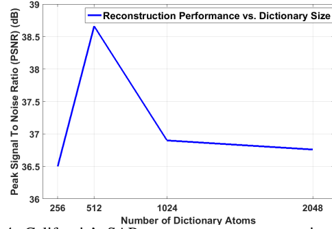
Figure 4: California's SAR measurement reconstruction. In this figure we examine the reconstruction performance of the active measurement as a function of the number of dictionary atoms used. As we may observe, the best performance is achieved when we use 512 dictionary atoms. Additionally, as the dictionary size increases above 512, the reconstruction quality decreases.
