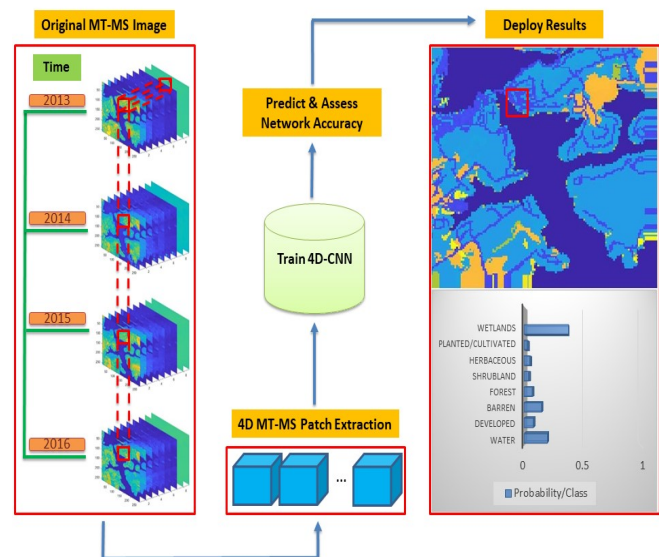
Fig. 1: The proposed method pipeline for the MT-RS land-cover classification task. Spatial patches are extracted across all available spectral bands and time instances of the MT-RS imagery, and subsequently fed to the proposed 4D-CNN system charged with the task of pixel-level classification.
