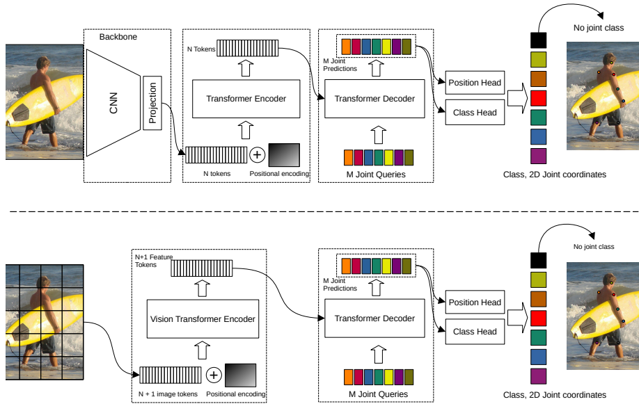
Fig. 1. The DETR model adapted for 2D human pose estimation (top) and our proposed model using Visual transformers (bottom). In our model, the cropped image of a person (bottom left), is split into N tokens of p \times p pixels (typically p is equal to 8 or 16 pixels). The tokens are processed by the transformer encoder (can be Deit or Xcit based). The output feature tokens ( N + 1 for the class token) are used as the memory tokens in the DETR based transformer decoder. The decoder input is M joint queries. M = 100 in our experiments. The Decoder outputs M prediction tokens which are processed by a classification and a regression head (FFNs). The output is 2D joint locations (range [0, 1] ) and class predictions.
