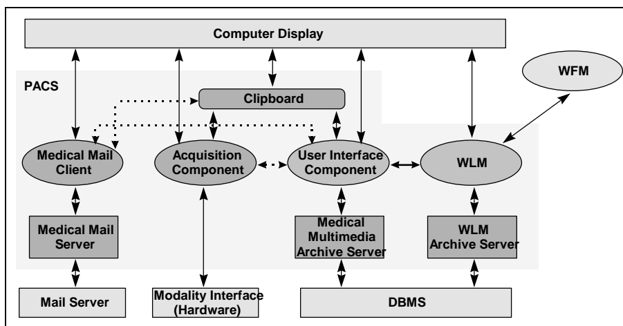
Figure 1. The PACS Architecture.
