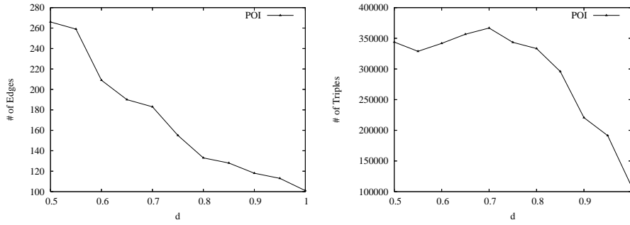
Figure 3: # of graph edges (left) and triples (right) for POI
