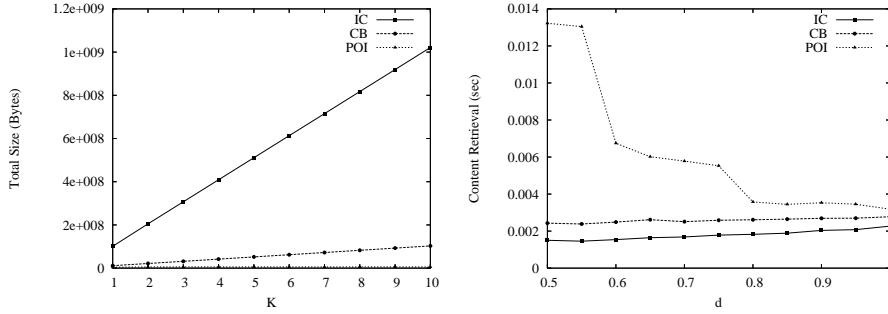
Figure 4: Storage space requirements (left) and retrieval costs (right) of IC, CB and POI
