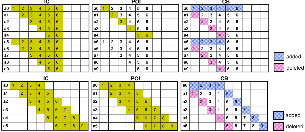
Figure 2: Best (upper) and worst (bottom) case for POI
