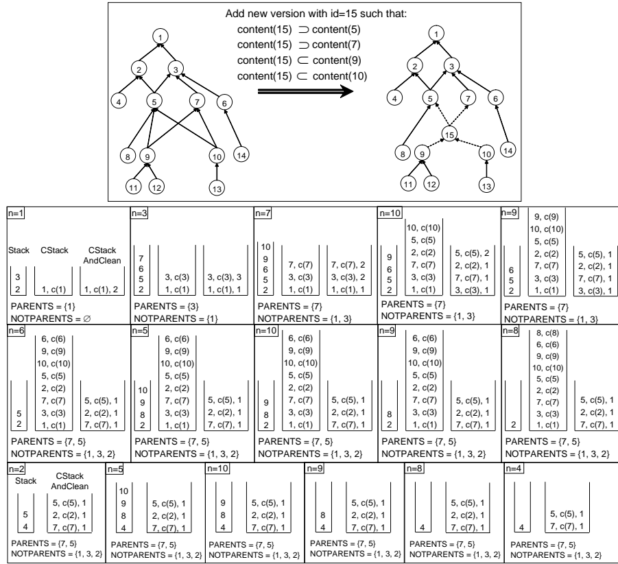
Figure 5: Example of adding a new version using Algorithm Insert POIDs
