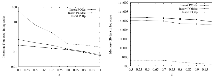
Figure 6: Comparison of Insert-POI implementations
