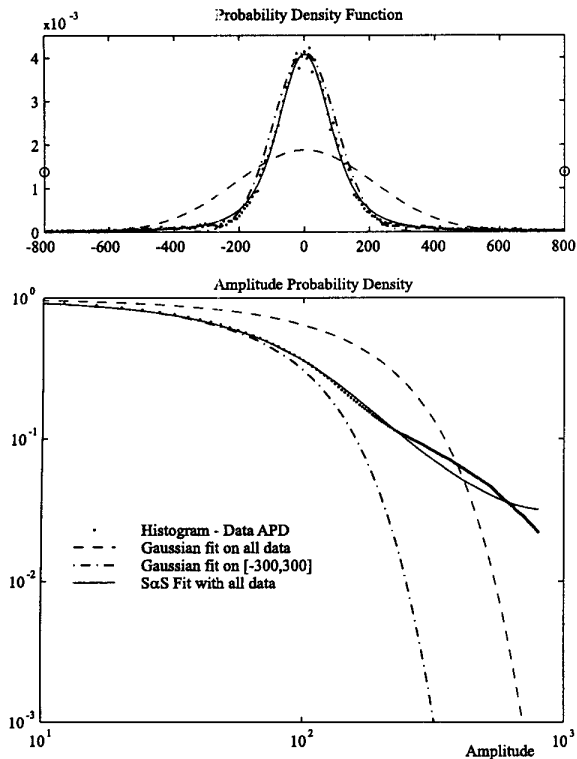
Figure 1: Comparison of the Gaussian, S\alpha S , and real data PDF and APD's.
